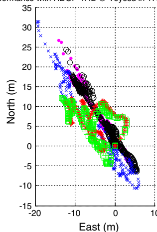
Fig. 9 Position errors with the Fraunhofer front-end and different receiver configurations in Toyosu, Tokyo. The horizontal dilution of precision (HDOP) is 4.42 in all positioning cases which indicates a poor satellite geometry
