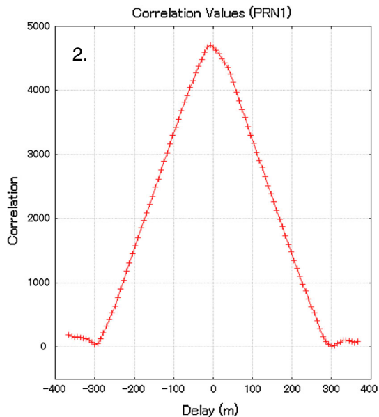
Fig. 8 Calculated C/N_0 of the experiment of urban canyon is shown in upper plot, and the correlation shape of the normal case and multipath effect are shown in lower plot
